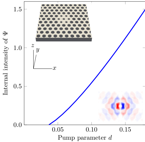
FIG. 8. (Color online) 3D calculation of a lasing mode created by a “defect” in a photonic-crystal slab [12]: a period- a hexagonal lattice of air holes (with a = 1 mm and radius 0.3 mm) in a dielectric medium with index n = \sqrt{\epsilon_c} = 3.4 with a cavity formed by seven holes of radius 0.2 mm in which a doubly degenerate mode is confined by a photonic band gap (one of these degenerate modes is selected by symmetry; see text). The gain has \gamma_{\perp} = 2.0 \text{ mm}^{-1} , k_a = 1.5 \text{ mm}^{-1} , and nonuniform pump D_0(\mathbf{x}, d) = f(\mathbf{x})d , where the pump profile f(\mathbf{x}) = 1 in the hexagonal region of height 2 mm in the y direction, and f(\mathbf{x}) = 0 outside that region and in all air holes. The slab has a finite thickness 0.5 mm with air above and below into which the mode can radiate (terminated by PML absorbers). The inset shows magnetic field H_z ( \sim \partial_x E_y - \partial_y E_x ) of the TE-like mode at the z = 0 plane.
